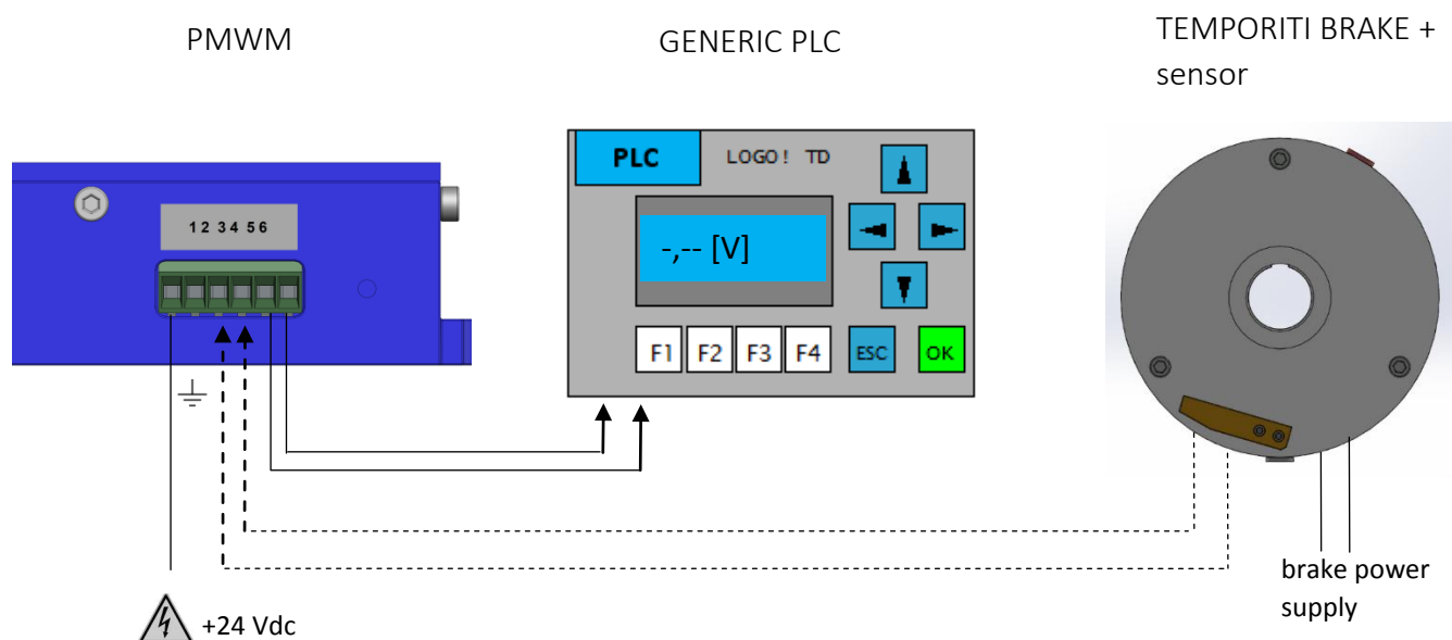
Fig. 1: Electrical connection
